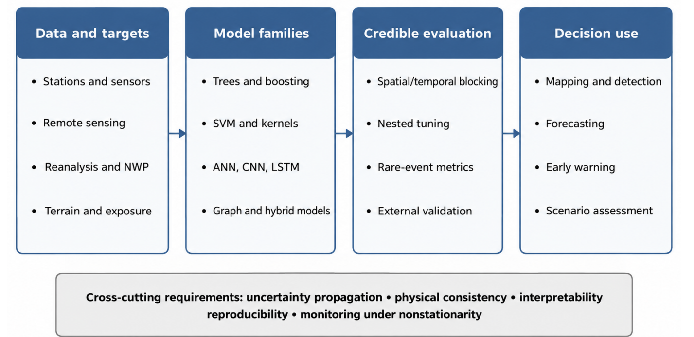
Figure 3 Cross-Hazard Modeling Pipeline. Credible Evaluation and Cross-Cutting Safeguards Connect Data-Driven Performance to Decision Use. NWP, Numerical Weather Prediction; SVM, Support Vector Machine; ANN, Artificial Neural Network; CNN, Convolutional Neural Network; LSTM, Long Short-Term Memory.
