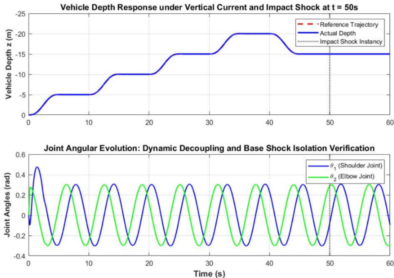
Figure 10 Kinematic Response of the Underwater Robot under Vertical Ocean Currents and a 10 N Impact Shock at T = 50 S: (Top) Vehicle Depth Tracking Performance; (Bottom) Joint Angular Evolution Verifying Dynamic Decoupling and Shock Isolation. Note that Both Controllers (Classical Smc and It2-Fsmc) Achieved Identical, Highly Precise Depth Trajectory Tracking; the Fundamental Superiority of the Proposed It2-Fsmc Lies Entirely in Generating a Chattering-Free Control Effort to Achieve This, as Previously Demonstrated in Figure 9.
