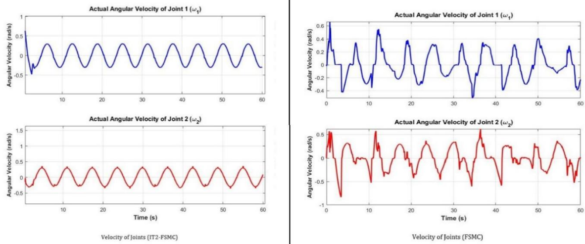
Figure 7 Angular Velocity Response of the Rigid Joints under Extreme Uncertainty
