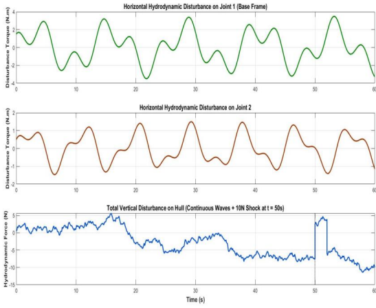
Figure 3 Simulated Hydrodynamic Disturbances. Time-Varying Ocean Currents Act on the Joints, and a Sudden 10 N Vertical Shock Is Applied to the ROV Base.
