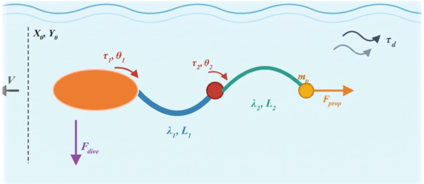
Figure 1 Schematic Diagram of the Flexible Structure of the Underwater Robot (ROV). It showing the global coordinate system (X_0, Y_0) , active thruster forces ( F_{prop} , F_{dive} ), joint control torques ( \tau_1 , \tau_2 ), and hydrodynamic disturbances ( \tau_d ).
