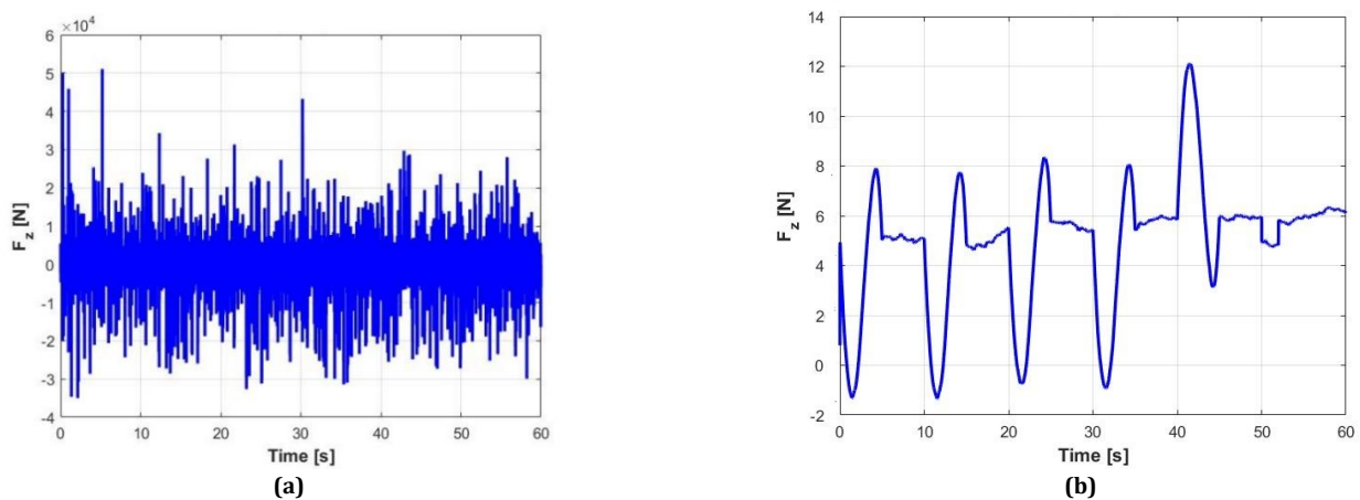
Figure 9 Comparative Analysis of the Thruster Control Effort ( F_z ) for the Rov Heave Axis under a 10 n Vertical Disturbance at t = 50 s: (a) Control Effort Generated by the FTSMC Exhibiting Severe Chattering; (b) Smooth Control Effort Generated by the Proposed IT2-FSMC to Mitigate Chattering.
