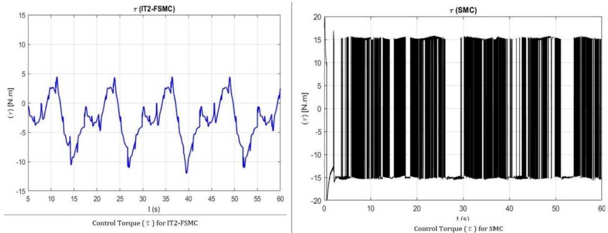
Figure 8 Comparative Analysis of the Applied Control Effort (Torque \tau ). The classical SMC exhibits severe high-frequency chattering, while the IT2-FSMC delivers a highly smooth and adaptive torque profile.
