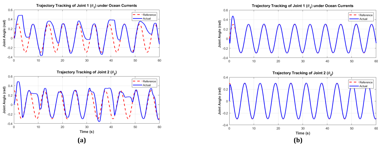
Figure 6 The Angular Trajectory Tracking of the Flexible Joints under 50% Parametric Uncertainty and Hydrodynamic Disturbances: (a) Failure of Joint Angle Tracking of Type-1 FSMC; (b) Successful Precise Tracking of the Proposed IT2-FSMC as Seen from the Figure.
